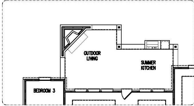
OPTIONAL OUTDOOR LIVING
